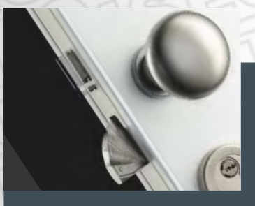
Multiblindo Motion EXIT Electronic Multipoint Lock
